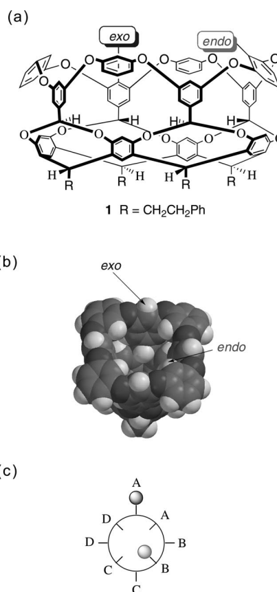
Figure 1. (a) Chemical structure and (b) space-filling model of cavitand 1 , showing the endo and exo positions. (c) Representation of a di-substituted cavitand to illustrate the nomenclature used (see text).
