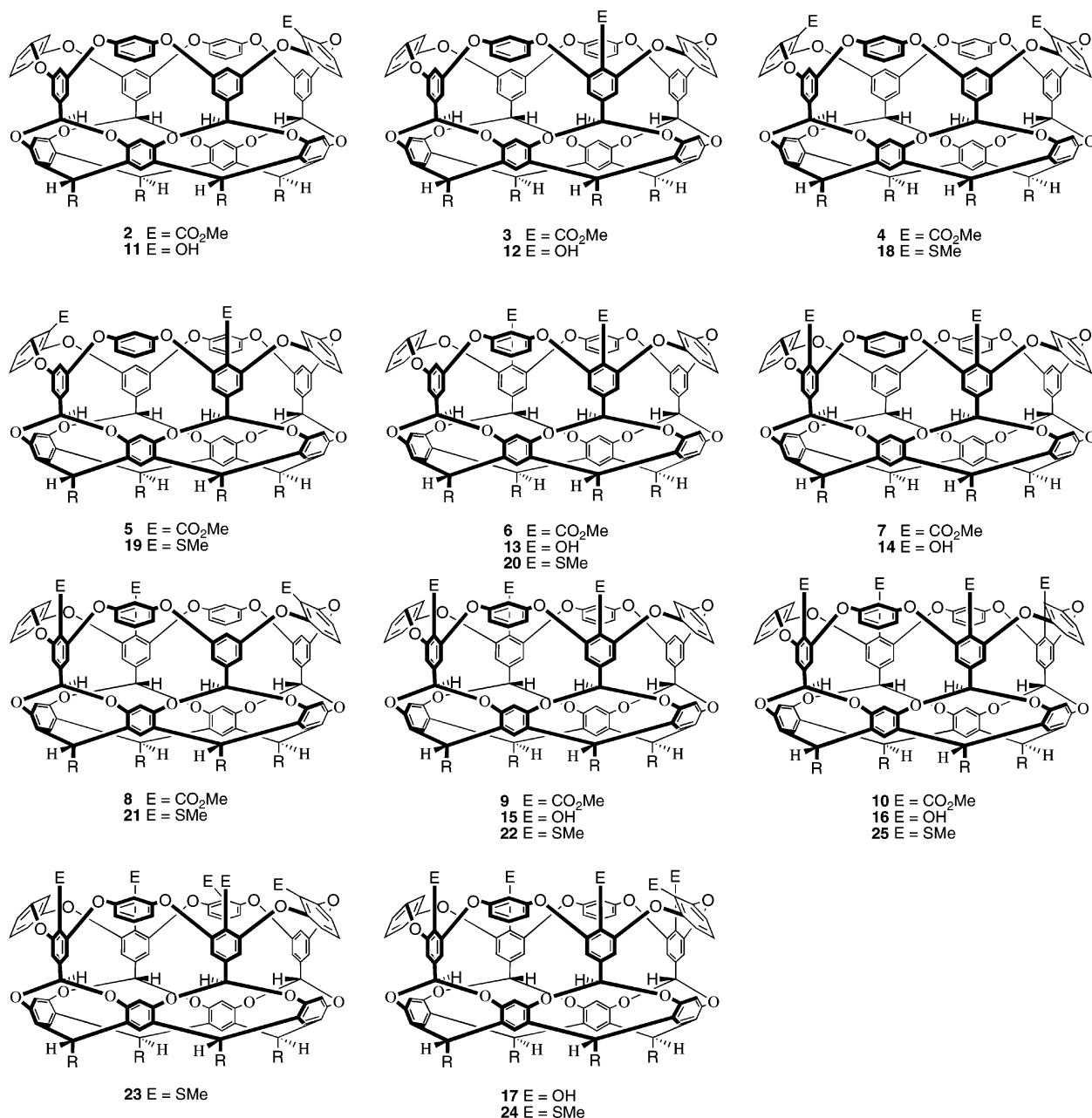
Figure 2. Chemical structures of products arising from this study.
