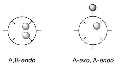
Figure 3. Rarely observed functionalization patterns.
